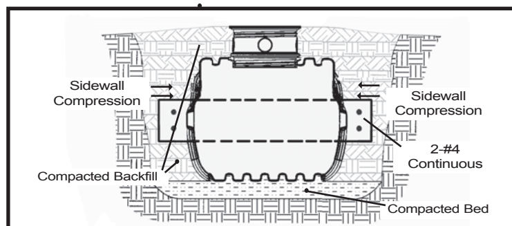
FIG.4 Backfilling
